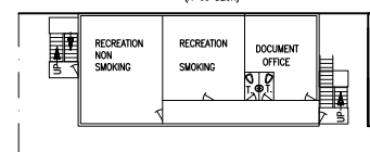
RECREATION DECK 1-ST LEVEL (A-60 DECK)
